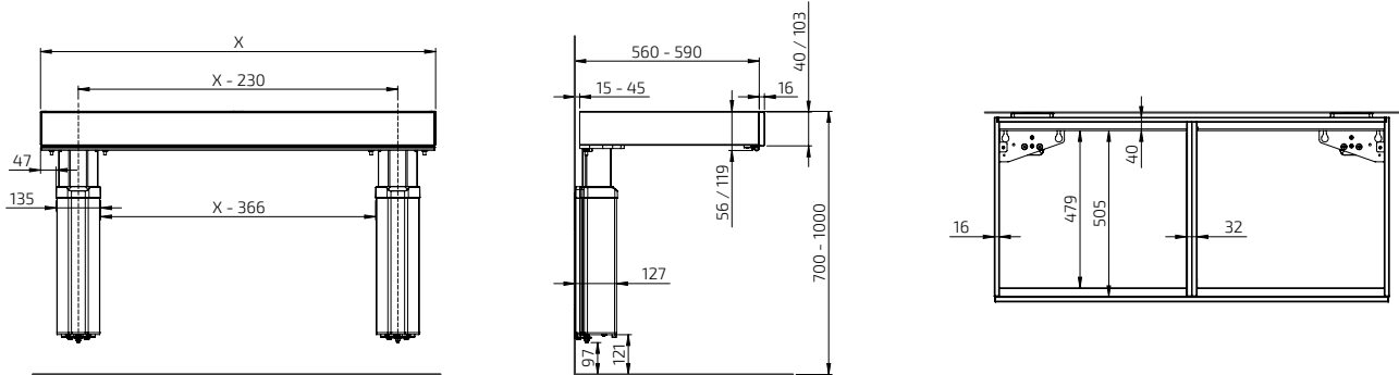
WALL-MOUNTED: 6300H/6300L
